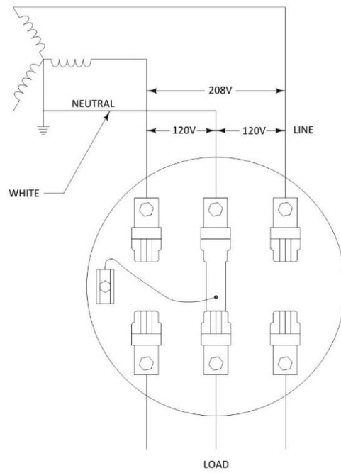
3-WIRE NETWORK 120/208 VOLT SINGLE PHASE SELF CONTAINED
