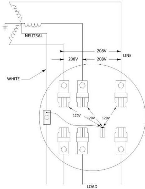
4 WIRE WYE 120/208 VOLT THREE PHASE SELF CONTAINED
