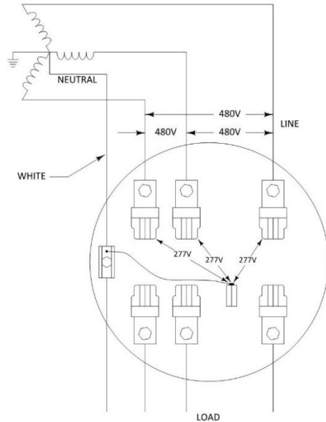
4 WIRE WYE 277/480 VOLT THREE PHASE SELF CONTAINED
