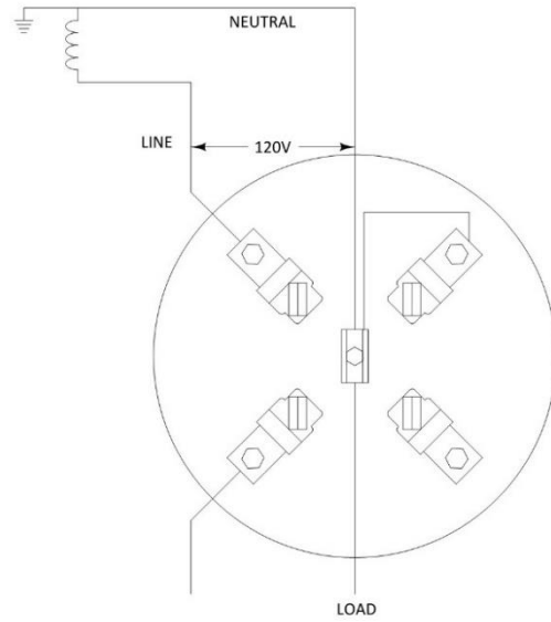
2-WIRE 120 VOLT SINGLE PHASE SELF CONTAINED
