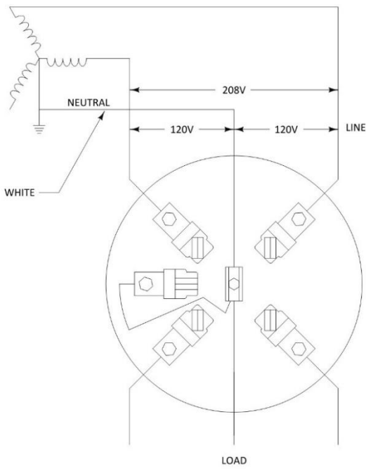
3-WIRE NETWORK 120/208 VOLT SINGLE PHASE SELF CONTAINED
