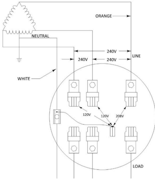
4-WIRE DELTA 120/240 VOLT THREE PHASE SELF-CONTAINED
