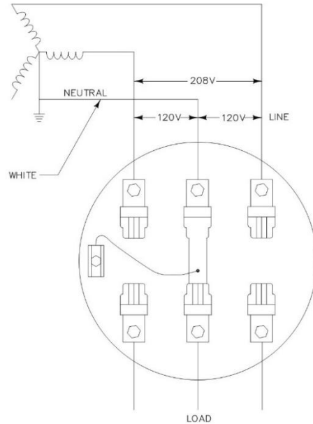
3 WIRE NETWORK 120/208 VOLT SINGLE PHASE SELF CONTAINED
