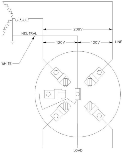
3 WIRE NETWORK 120/208 VOLT SINGLE PHASE SELF CONTAINED
