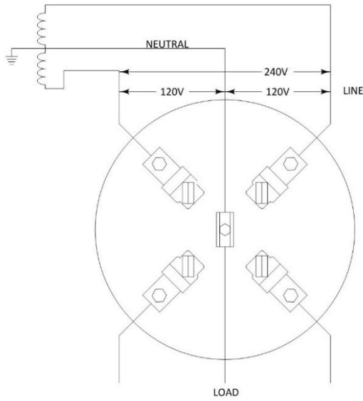
3-WIRE 120/240 VOLT SINGLE PHASE SELF CONTAINED
